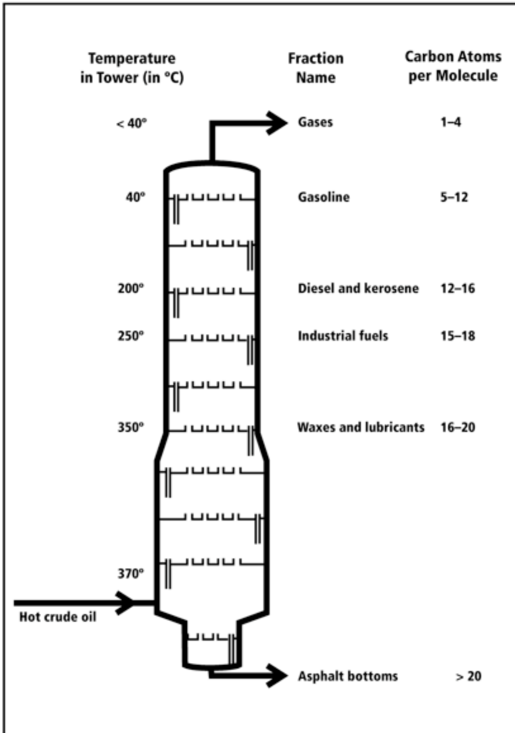
Diagram of a Fractional Distillation Tower
